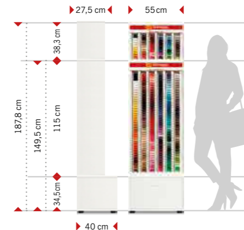
SVK A 60/22
